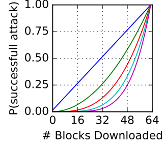
(b) The probability that the attacker is successful given a fixed amount of download trials. Super blocks count (left→right): — 1, — 2, — 3, — 4, — 5.
