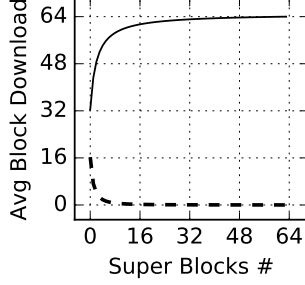
(a) The average number of blocks that an attacker has to download (—) and its rate of change (---).
